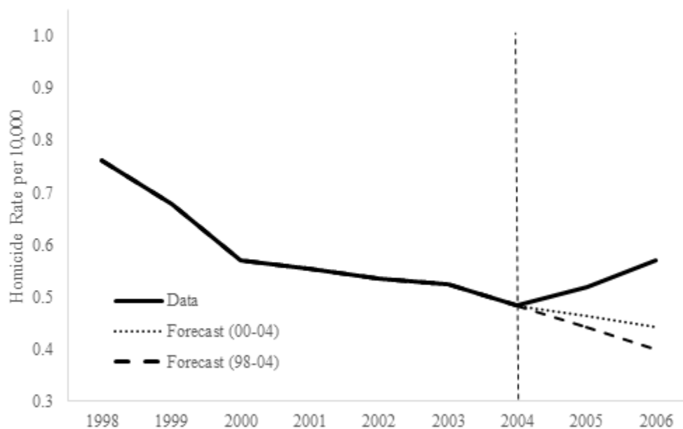
Figure 3: Firearm Homicide Rate and Counterfactual Trends
