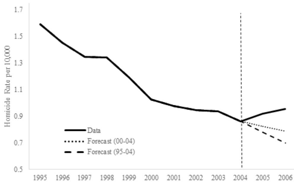
Figure 2: Overall Homicide Rate and Counterfactual Trends
